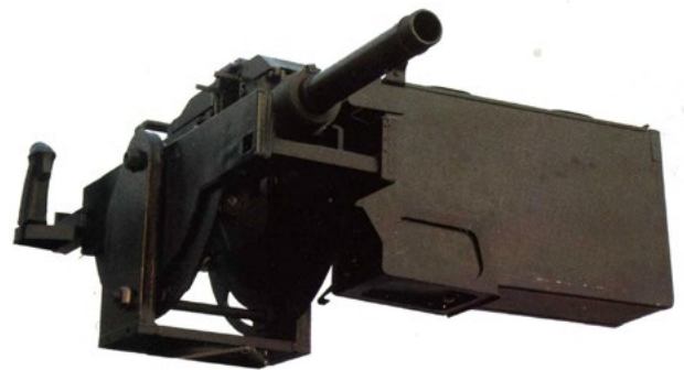
Image of vehicle mounted 38mm automatic grenade launcher taken from marketing material by No.208 Research Institute of China Ordnance Industries (right) and (left) product on display at China Police 2014 . Photograph: © Robin Ballantyne/Omega Research Foundation.
