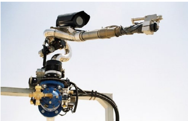
Images of water restraint system (WRS) taken from Beit Alfa Technologies website
